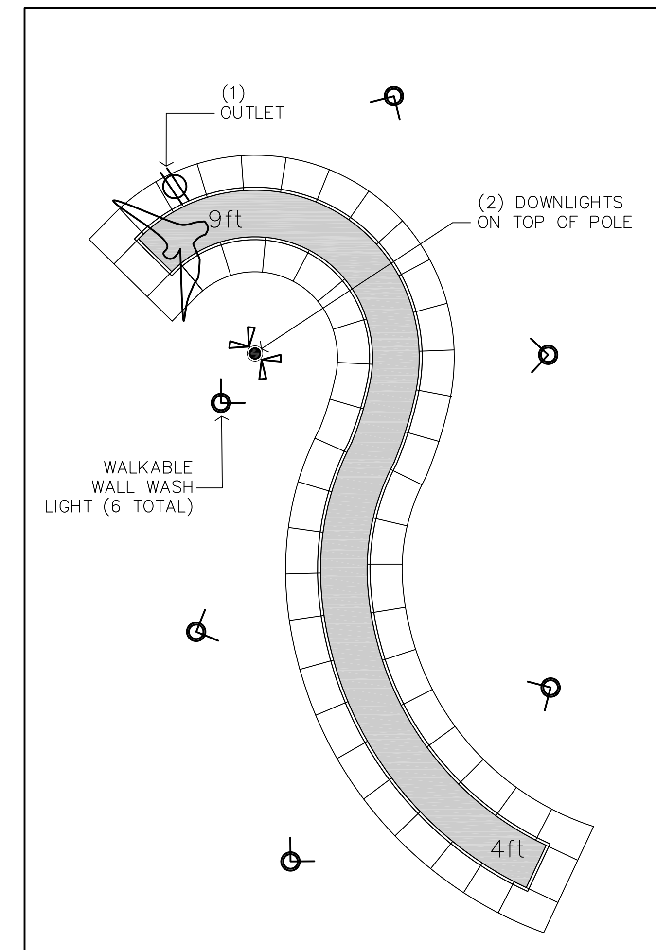
LIGHTING LAYOUT SCALE: 1/4" = 1'-0"
