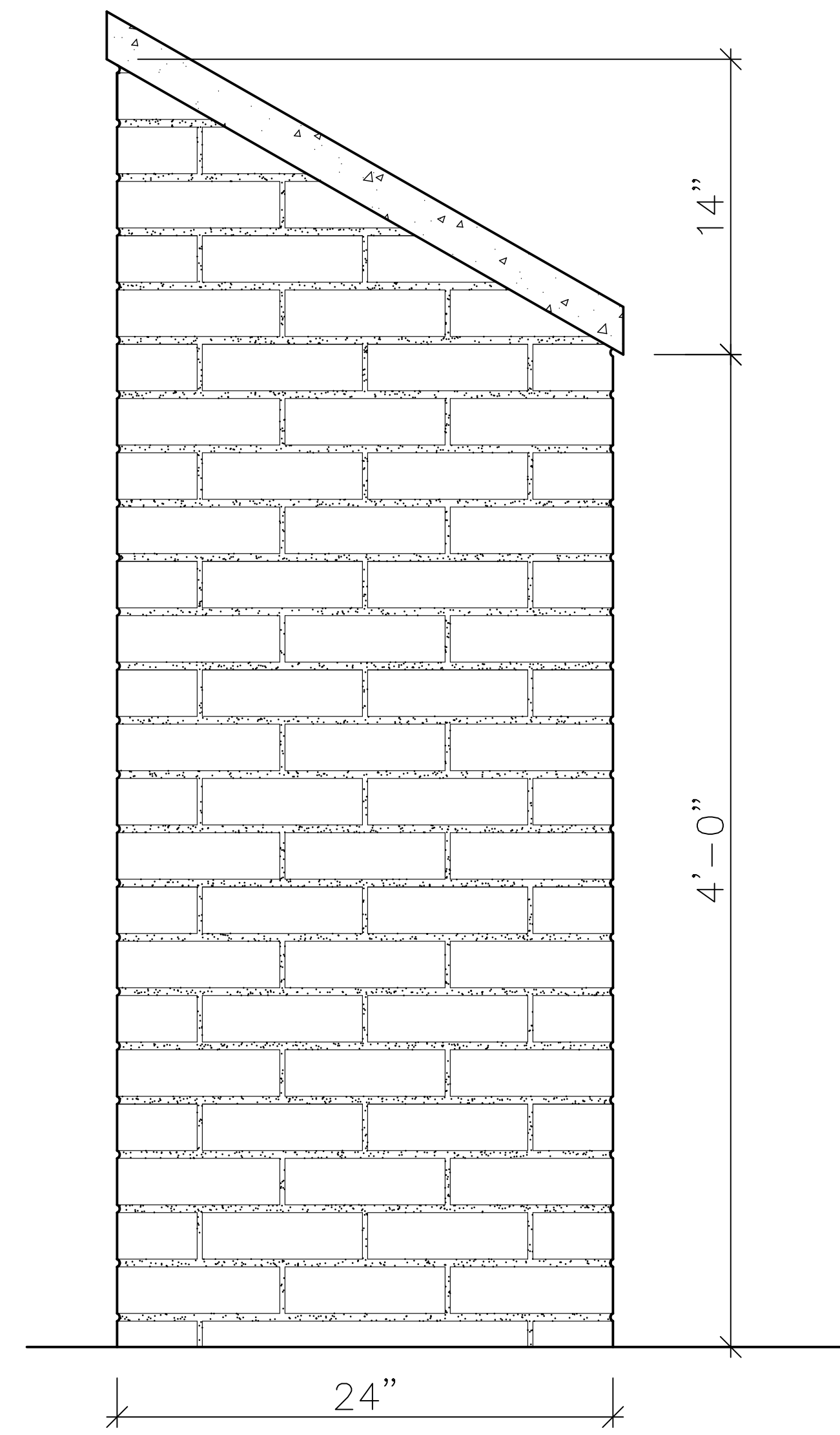
WALL END ELEVATION - LOW START SCALE: 2" = 1'-0"
