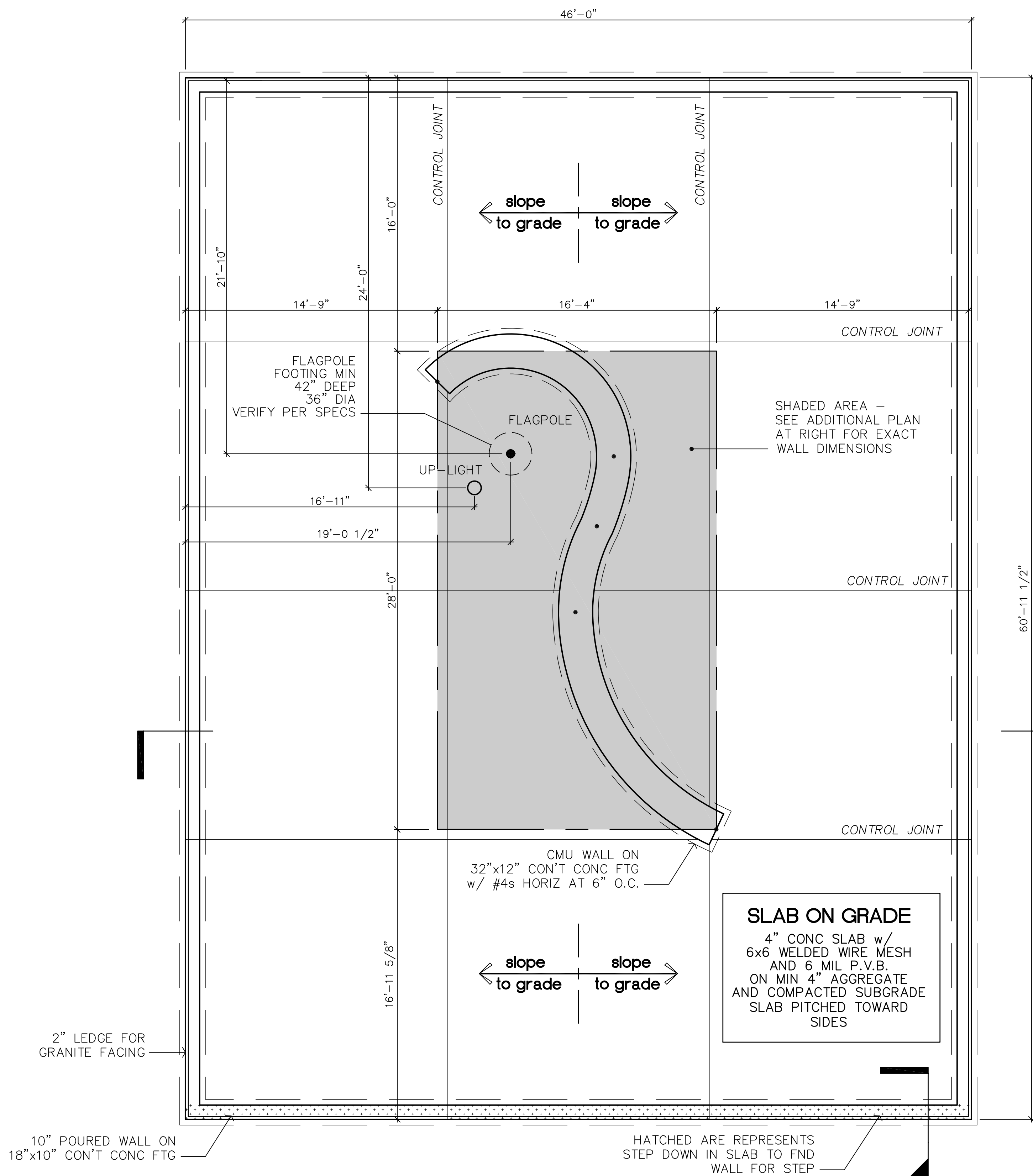
FOUNDATION / SLAB ON GRADE PLAN SCALE: 1/4" = 1'-0"
