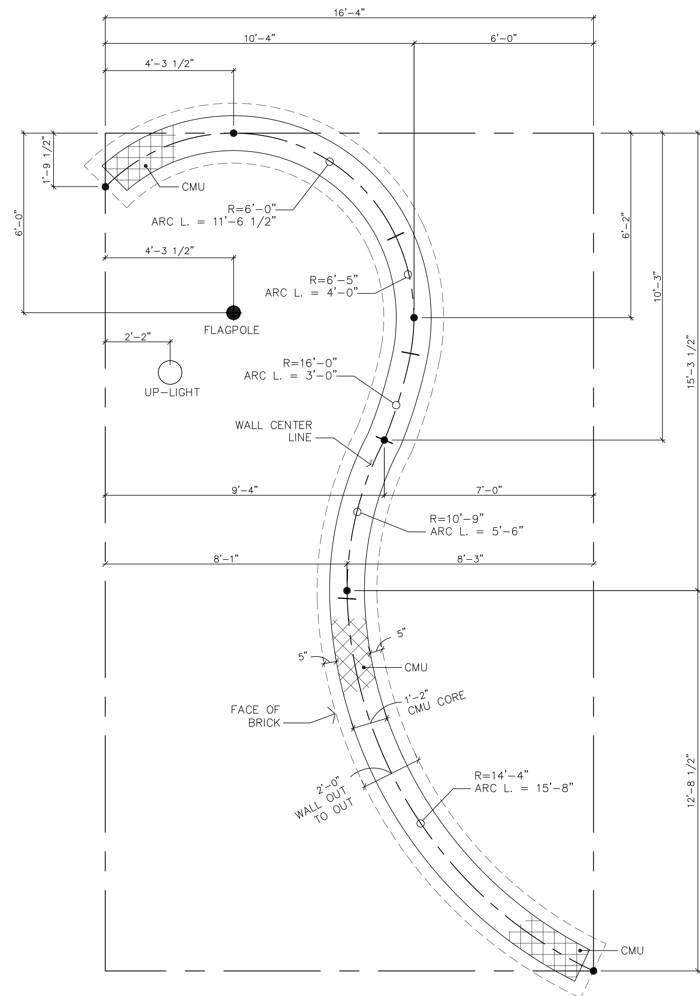
WALL DIMENSIONS SCALE: 1/2" = 1'-0"
